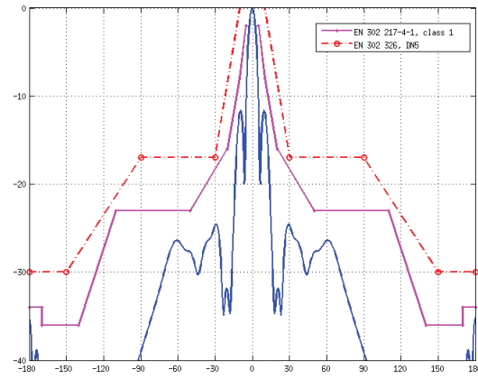
E-Plane Specs
