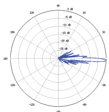
Horizontal Elevation
